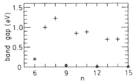
FIG. 3. The energy band gap as a function of the number of hexagons on the circumference for tubules B(1,0)n . Symbols \odot and + represent the classes of narrow-gap and moderate-gap semiconductors, respectively.
