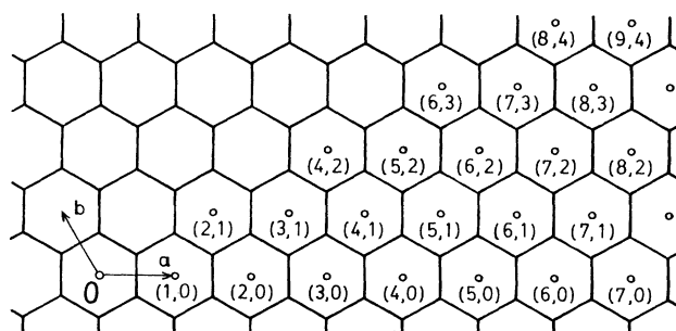
FIG. 1. A monatomic layer of graphite. Vectors \mathbf{a} and \mathbf{b} are unit vectors of the two-dimensional lattice. The coordinates of the lattice points are shown in the figure, which are useful to distinguish the crystal structures of tubules.
