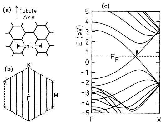
FIG. 4. (a) The geometric configuration for tubule B(2,1)n . (b) The first Brillouin zone of a graphite sheet (dashed line), and the wave vectors allowed by the periodic boundary condition along the circumference for n=4 (solid lines). Open circles show the points where the bonding and the antibonding \pi bands are degenerate in the tubule. (c) Band structure of B(2,1)6 . The X point has a wave number near \sqrt{3}\pi/a . The arrow shows a wave vector corresponding to the K point.
