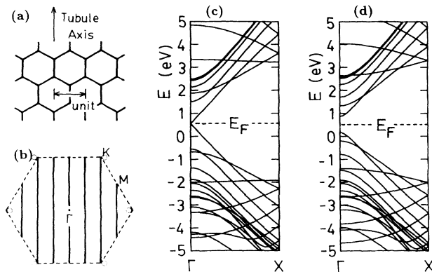
FIG. 2. (a) The geometric configuration for tubule B(1,0)n . "Unit" is the construction unit along the circumference, denoted by (1,0) . The notation B(1,0)n means that the tubule has n construction units on the circumference. (b) The first Brillouin zone of a graphite sheet (the region surrounded by the dashed line), and the wave vectors allowed by the periodic boundary condition along the circumference for n=6 (solid lines). Open circles show the points where the bonding and the antibonding \pi bands are degenerate in the tubule. Band structure of (c) B(1,0)12 and (d) B(1,0)13 . The X point has a wave number near \pi/a , with a the graphite in-plane lattice constant. Two bands stick together at the X point due to the screw symmetry.
